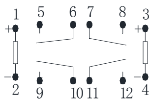
2 coil non-latch:4a 2 coil latch:4a
