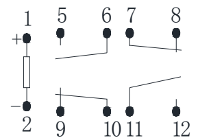
1 coil non-latch:2a2b 1 coil latch:2a2b
