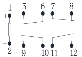
1 coil non-latch:3a1b 1 coil latch:3a1b
