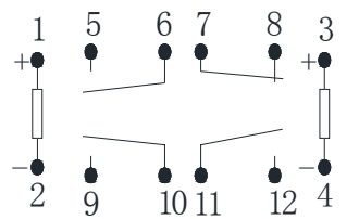
2 coil non-latch:3a1b 2 coil latch:3a1b
